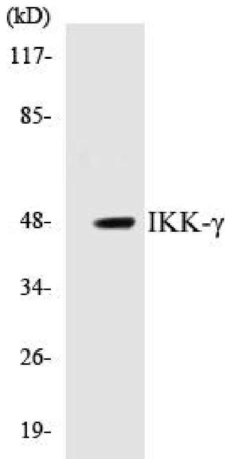
Figure 2. Western blot analysis of extracts from HepG2 cells, using IKK-gamma (Ab-31) Antibody.
